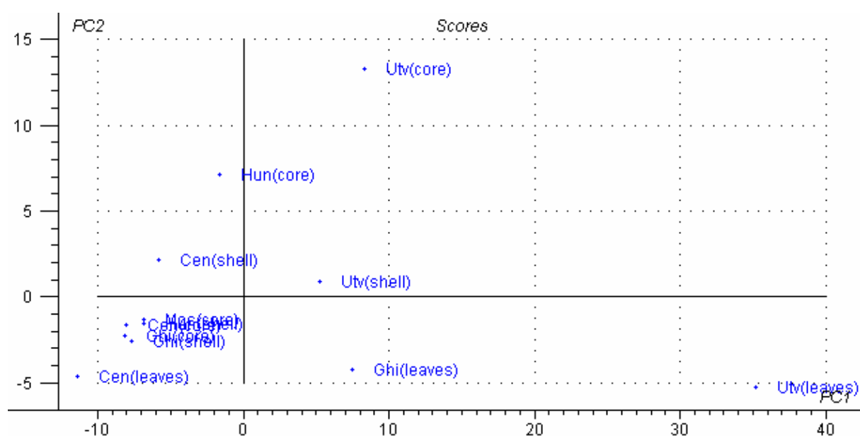
Fig. 7. Score plot for trace element data from PCA analysis
