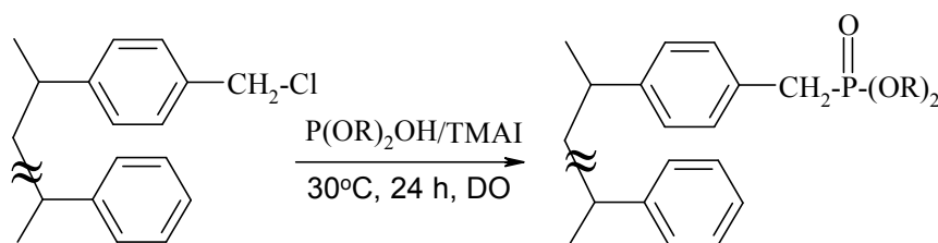
Fig. 1. Michaelis-Becker polymer-analogous functionalization reaction. Phosphite used: (CH 3 O) 2 POH, (C 2 H 5 O) 2 POH, (i-C 8 H 17 O) 2 POH, (C 2 H 5 -C 6 H 12 O) 2 POH
