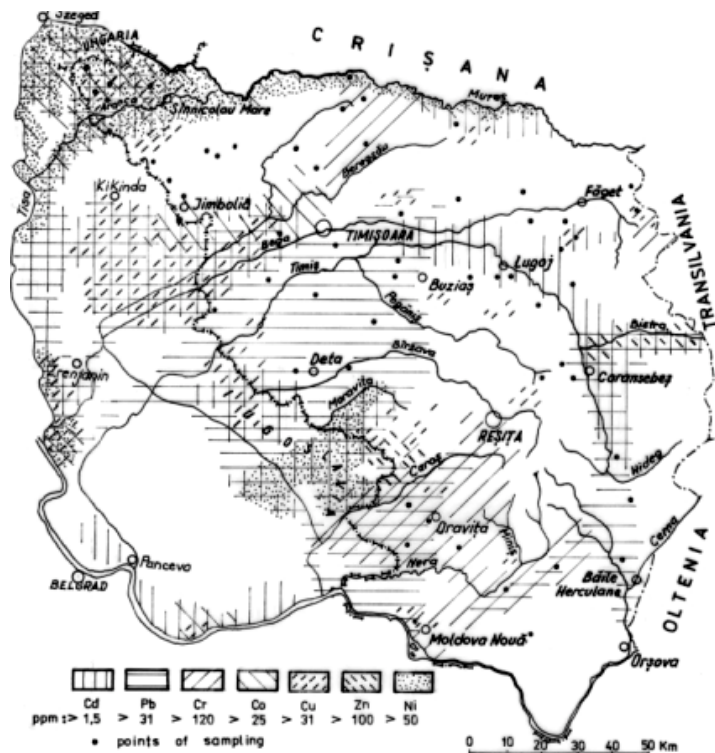
Fig. 2 Values of attentions of the heavy metals concentration in the soils of the Ethno-historical Banat
